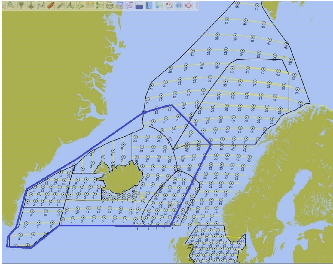
Maps shows proposed sampling stations and survey tracks for all nations participating in the IESSNS 2020. Geographical work area of the Icelandic vessel is within the area defined by the blue polygon. Locations of surface trawl stations, CTD and plankton sampling (open circle with a dot in centre) and survey tracks (yellow solid lines).
