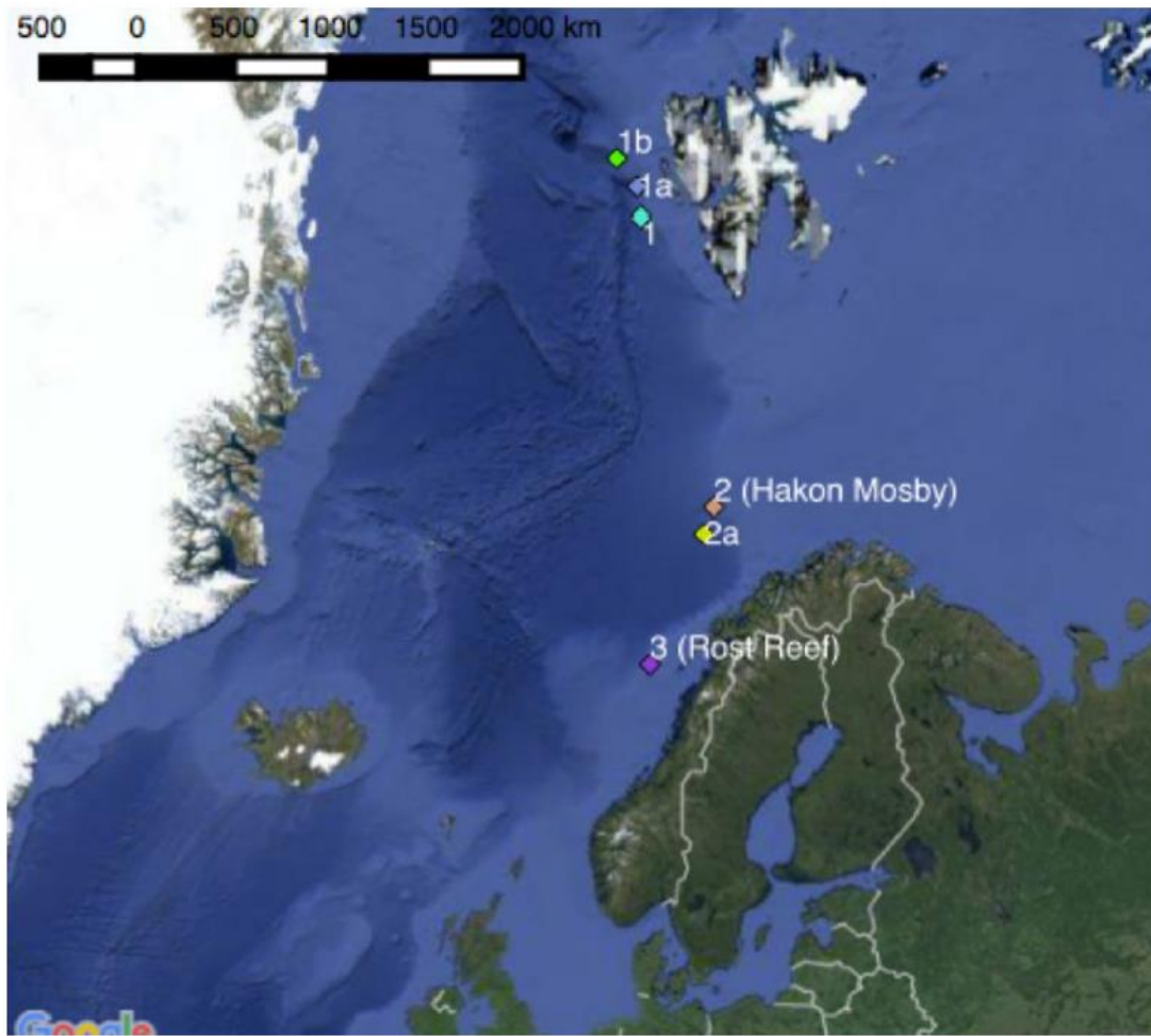
Fig. 1: Working areas of R/V HEINCKE cruise HE493. Proposed work areas in the Norwegian EEZ include the Røst reef.
