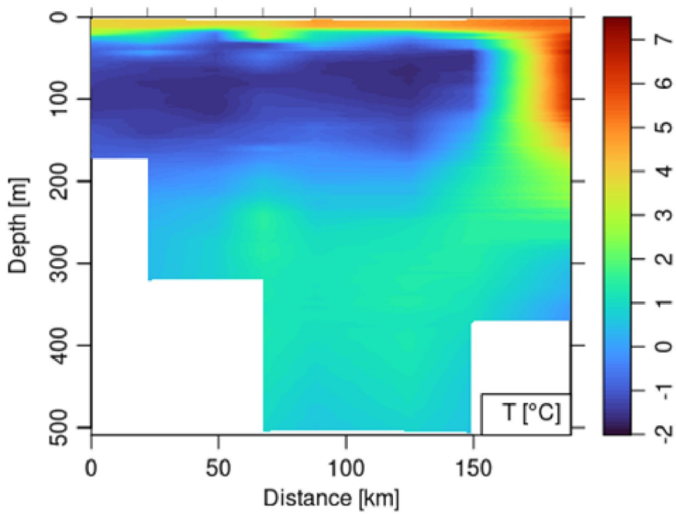
Figure 15: Temperature profile down to 500 m along transect B crossing Denmark Strait.
