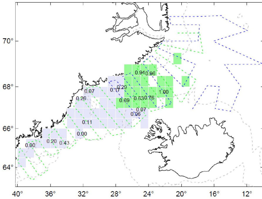
Figure 5: Proportion of mature capelin at each trawl station.
