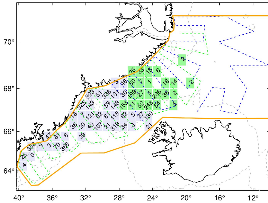
Figure 4: Capelin distribution as relative density of acoustic backscatter during the survey.
