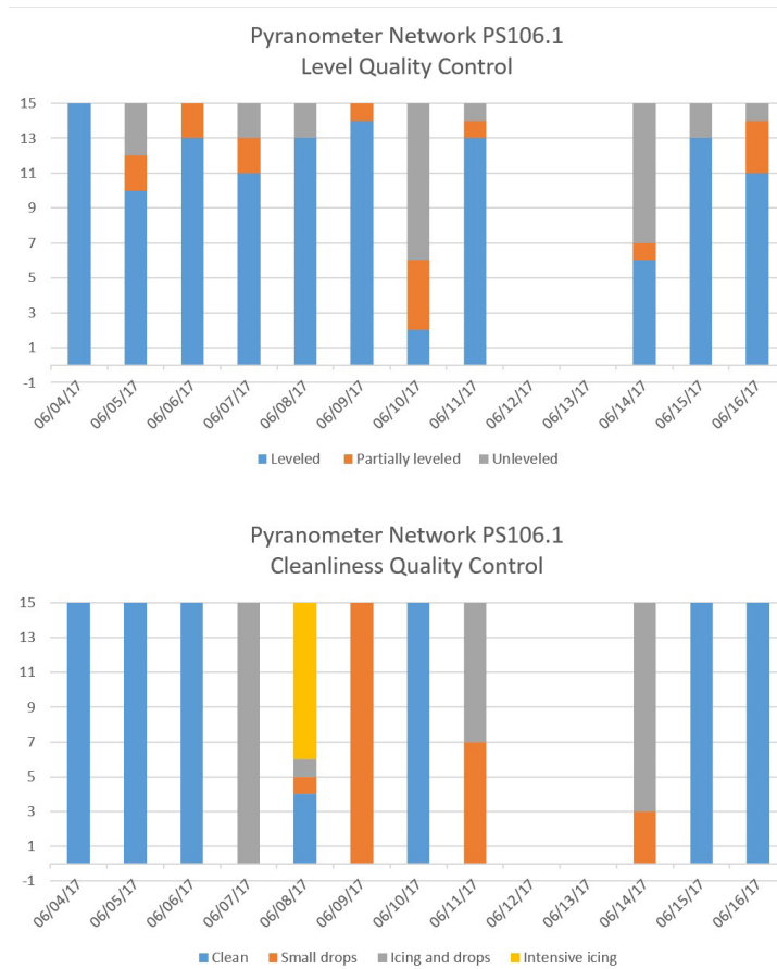
Fig. 3.14: Quality control of pyranometer. The upper plot shows the level quality and the bottom plot the cleanliness quality.
