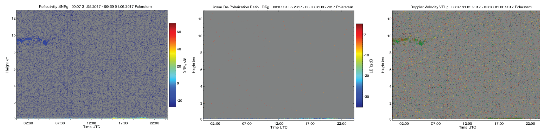
Fig. 3.10: Profile of reflectivity (left), linear depolarization ratio (middle) and Doppler velocity (right) for May 31, 2017
