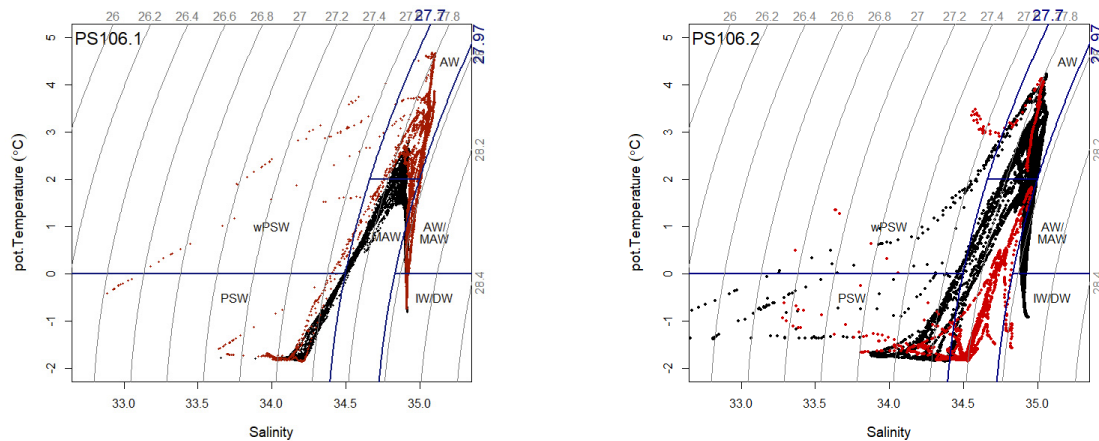
Fig. 9.7: Potential temperature/salinity diagram for all CTD/RO data measured during PS106/1 (left) and PS106/2 (right). Curved isopycnals indicate the potential density anomaly ( \sigma_{\theta} ; \sigma_{\theta} ), and denser water masses from left to right. Classification of the encountered water masses during PS106/1 mainly follow Rudels et al. (2000) as indicated by labels. Blue isolines in both diagrams indicate temperature ( q=0 and 2^{\circ}\text{C} ) and density ( \sigma_{\theta}=27.7 and 27.97 ) values crucial for these definitions. For PS106/1 (left) black dots show the casts during ice-floe drift and red dots all other casts. For PS106/2 (right) red dots show Barents Sea measurements and black dots all other casts.
