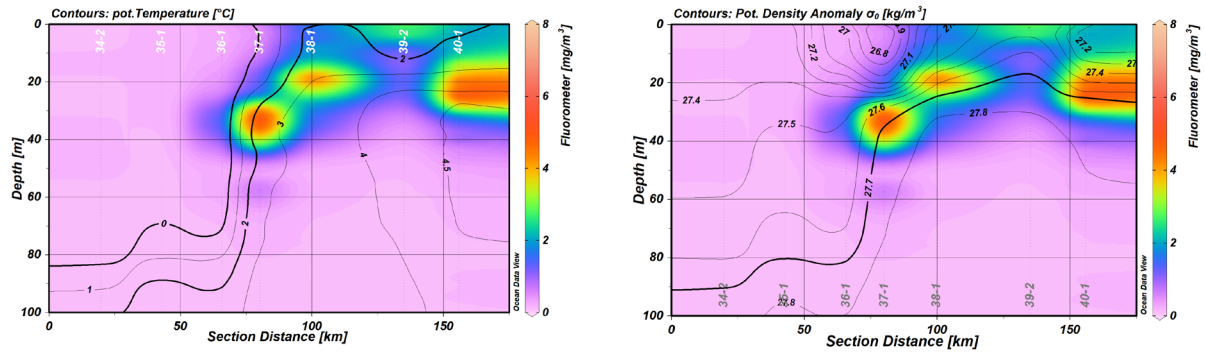
Fig. 9.11: Contoured sections of fluorescence overlaid by potential temperature (left) and density anomaly s_q (right), for the upper 100 m of stations 34-40. The maximum fluorescence values are found in the pycnocline within the relatively warm AW/wPSW, cf. the TS-diagram in Fig. 9.7. The full-depth temperature and salinity distributions are shown as sections in Fig. 9.12.
