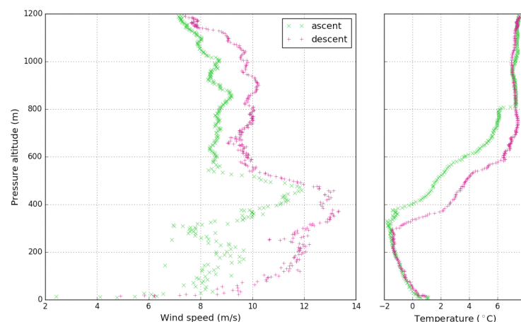
Fig. 3.20: Vertical profile of wind speed and temperature (raw data of hotwire anemometer package) of 28_TBT_1 with strong wind below a temperature inversion
