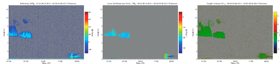
Fig. 3.11: Same as Fig. 3.11 but for June 8, 2017
