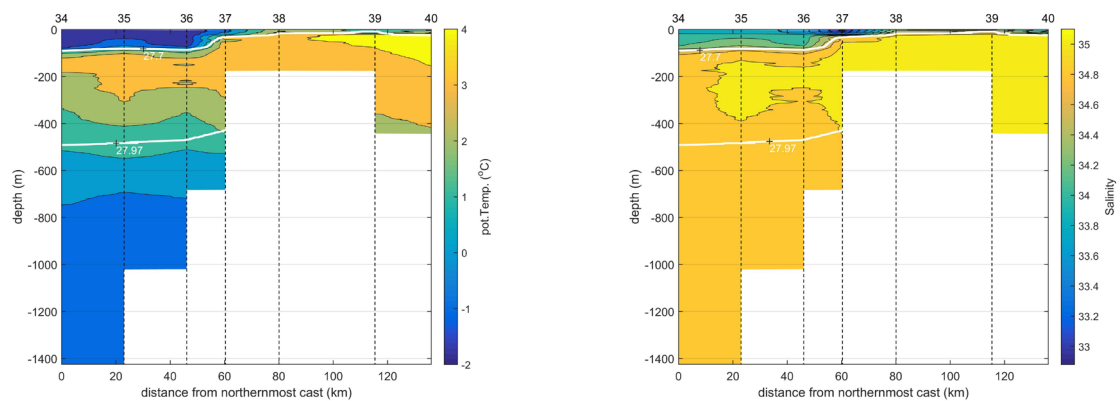
Fig. 9.12: Potential temperature (left) and salinity (right) across the shelf as measured during the transect of PS106/1. White lines show the sigma 27.7 and 27.97 isopycnals, respectively, cf. the TS-diagram in Fig. 9.4. Dashed vertical lines indicate the location of the casts (top labels), travelling from the north towards the shelf slope in a knee-shaped path as shown by Fig. 9.2.
