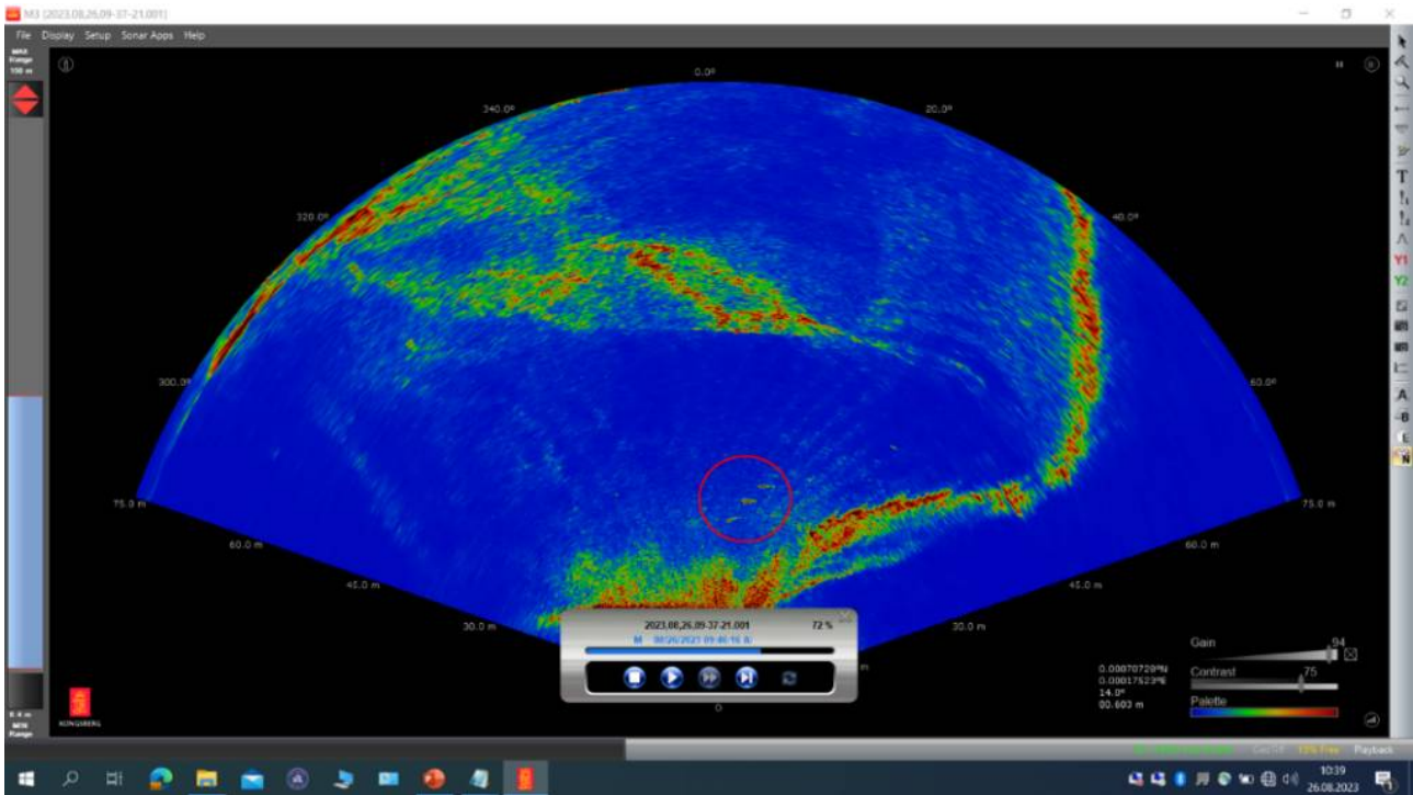
Figure 13. Screen dump from M3 sonar on 26.08.23 from inside the purse seine from Cast 3. The three BFT are circled in red. The larger and elongated scatters correspond to the purse seine net. Transducer located ca. 10 m from net wall with a sampling range of 75 m.
